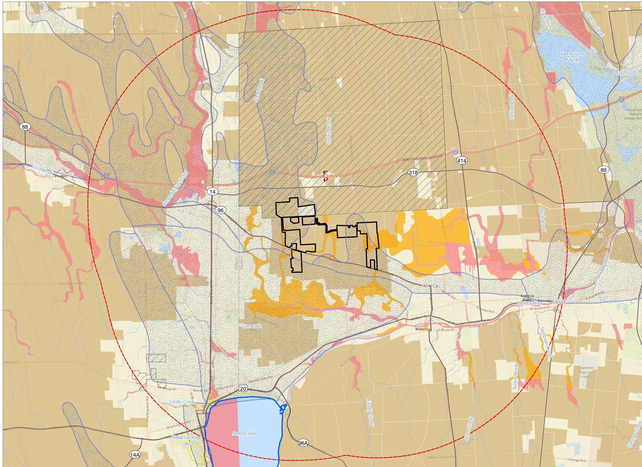
Figure 3-8. Specially-Designated Areas
