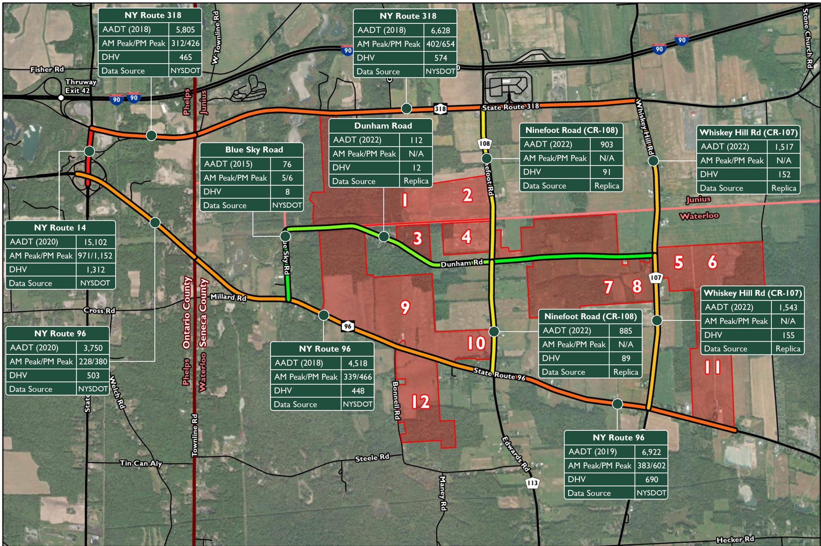
Figure No. 16- 4 Traffic Volumes
